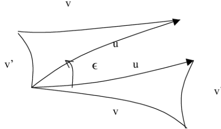
Figure 9: Varicak’s hyperbolic representation
